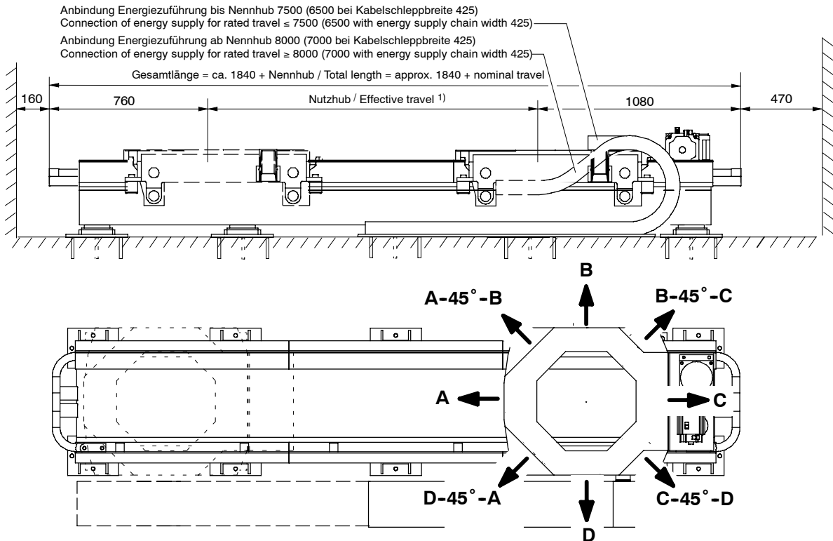
A, B, C, D = Robotermontagevarianten / Robot mounting variants
